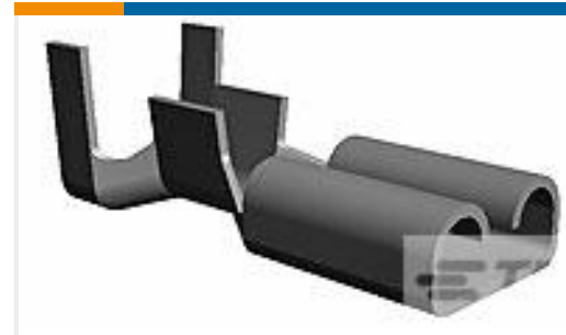
TE 零件编号1217129-1 FASTON 187 RECEPTACLE 24-20 AWG TPBR
